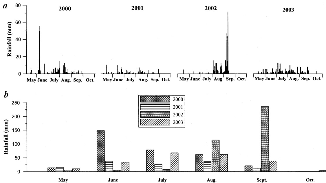
Figure 2. (a) Daily rainfall and (b) monthly rainfall observed near the snout of Gangotri Glacier (Bhojwasa, 3800 m) during summer seasons 2000 to 2003.
